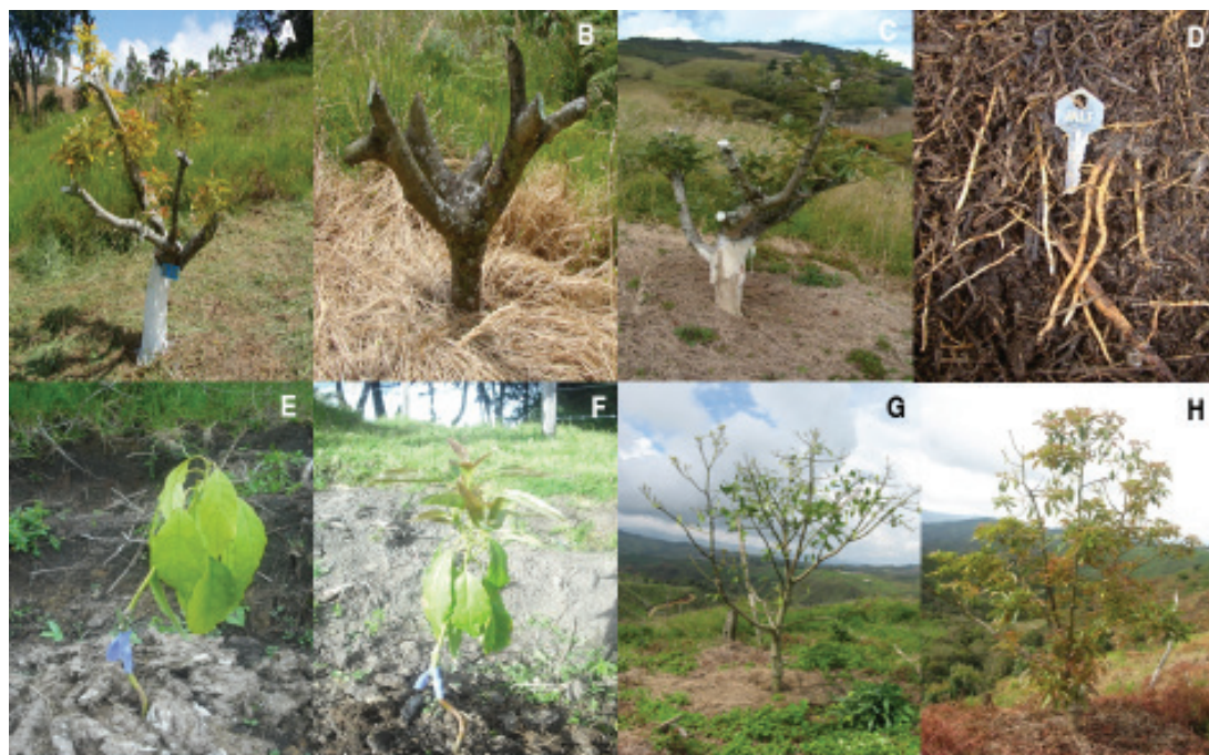
Figure 7. Results of management practices in avocado wilt complex. A. New leaf buds after performing severe pruning; B. Dead plant after performing severe pruning; C. Recovery of plant infected with P. citricola after performing surgery and complementary treatment; D. Induction of viable roots in plants with added mulching; E, F. Seedling infected with P. cinnamomi , and recovery after implementation of integrated management strategy; G, H. Adult infected with P. cinnamomi , and recovery after implementation of integrated management strategy. The photos are representation of results associated with AWC management under assays in field developed by the author.
