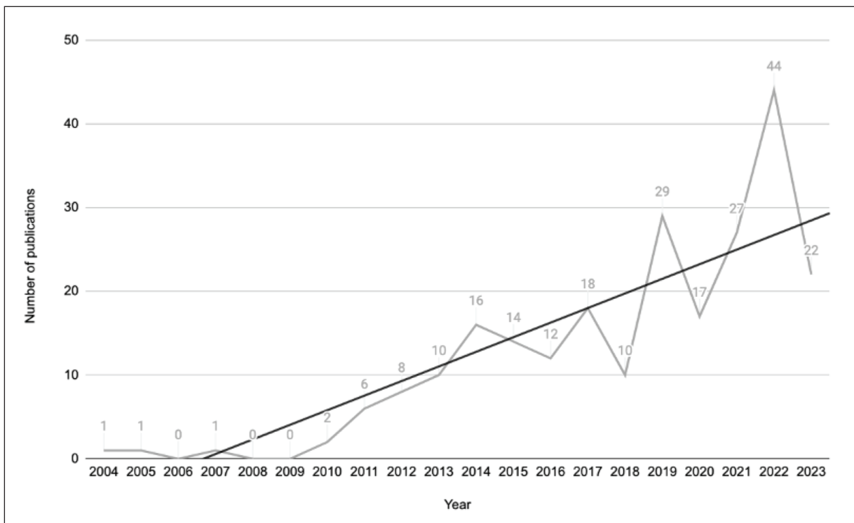
Figure 1. Annual publications.
