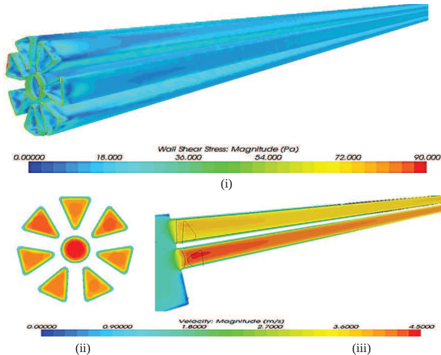
Figure 3. Membrane simulation results (i) wall shear stress for TSS 10 g/L, (ii) sectional velocity for TSS 10 g/L, (iii) velocity profile along the membrane for TSS 10 g/L.
