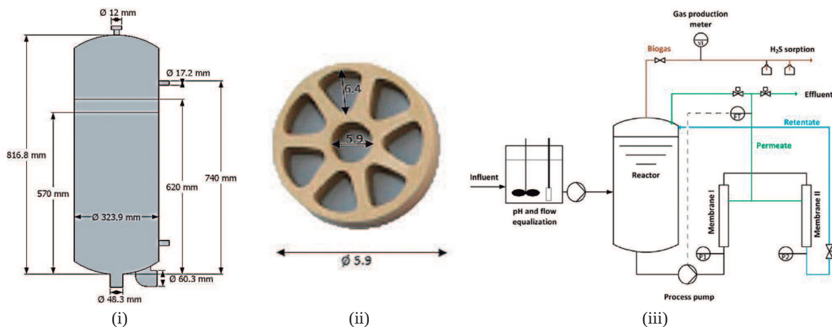
Figure 1. (i) Bioreactor, (ii) membrane (units in mm), (iii) AnMBR schematic flow diagram. Source: Own work.
