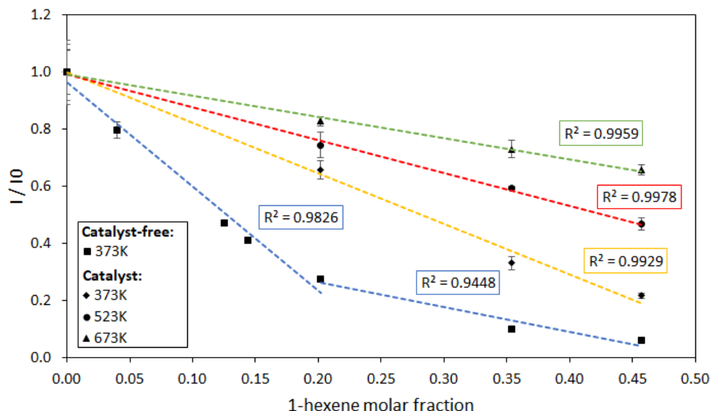
Fig. 8. Variation in fractional transmission ( I/I_0 ) as a function of the molar fraction of 1-hexene at different temperatures and in the presence and absence of a catalyst Source: Created by the authors.
