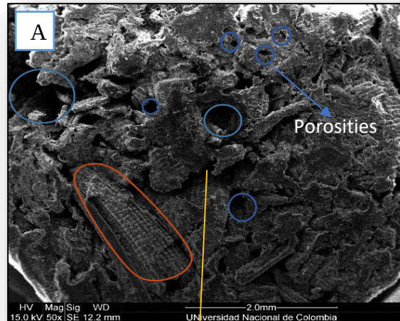
Test Specimen: Rice Husk Particleboard - External Section
