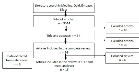
Figure 1 Search Flowchart
