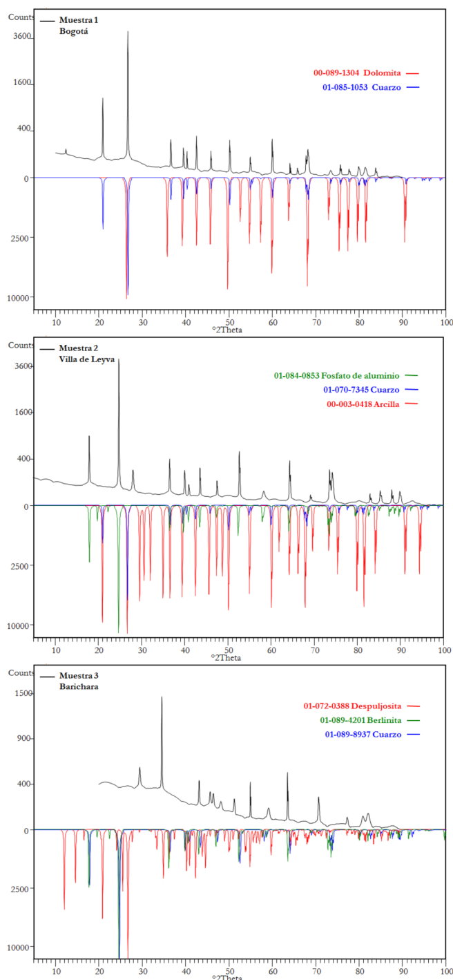
Fig 2. FTIR spectra and X-ray diffraction patterns of samples of mortars from the Casa Hacienda el Otoño in Bogotá (M1), Claustro de San Francisco in Villa de Leyva (M2) and House in Barichara (M3).
