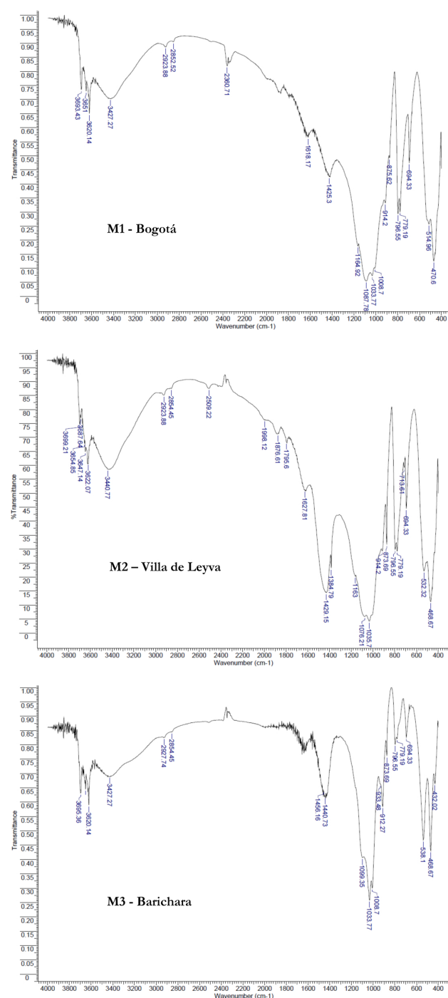
Fig 2. FTIR spectra and X-ray diffraction patterns of samples of mortars from the Casa Hacienda el Otoño in Bogotá (M1), Claustro de San Francisco in Villa de Leyva (M2) and House in Barichara (M3).
