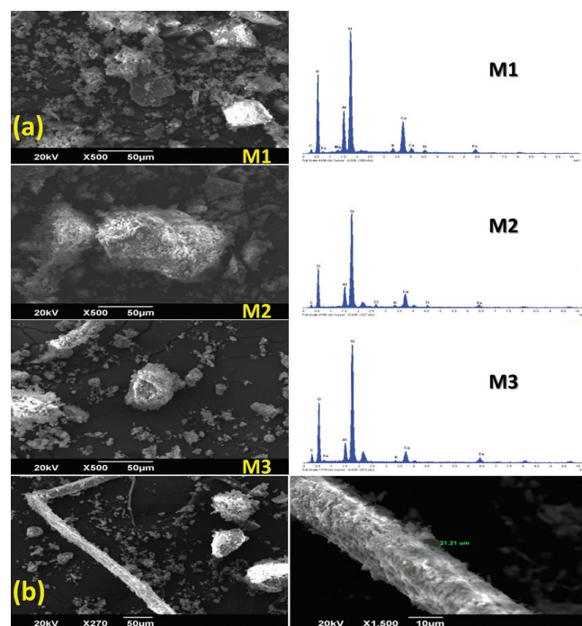
Fig 3. (a) SEM images and EDX spectra of mortar samples from the Casa Hacienda el Otoño in Bogotá (M1), Claustro de San Francisco in Villa de Leyva (M2) and House Barichara (M3). (b) SEM images of fibers found in mortars.
