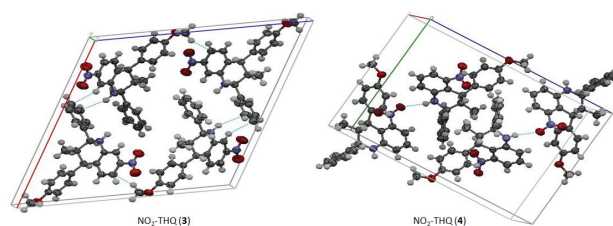
Fig. 4. Perspectives drawing of the packing arrangement in nitro-regioisomers THQ (3) and (4). Dashed lines indicate the intermolecular van der Waals interactions.
