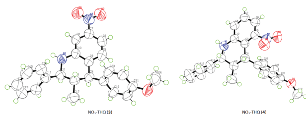
Fig. 3. The molecular structures of 7-nitro (3) and 5-nitro (4) tetrahydroquinolines, showing the atom-label scheme. Displacement ellipsoids are drawn at the 50% probability level (Farrugia 1997).
