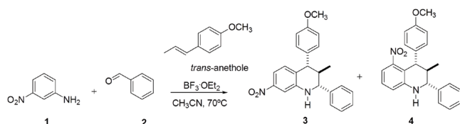
Fig. 1. Synthesis of nitro-regioisomers of tetrahydroquinolines using the three-component imino Diels-Alder reaction.
