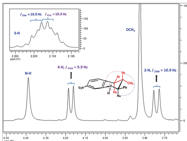
Fig. 2. Coupling between 3-H proton and 2-H and 4-H protons in ^1\text{H} RMN spectra of cis -4-(4-methoxyphenyl)-3-methyl-7-nitro-2-phenyl-1,2,3,4-tetrahydroquinoline.
