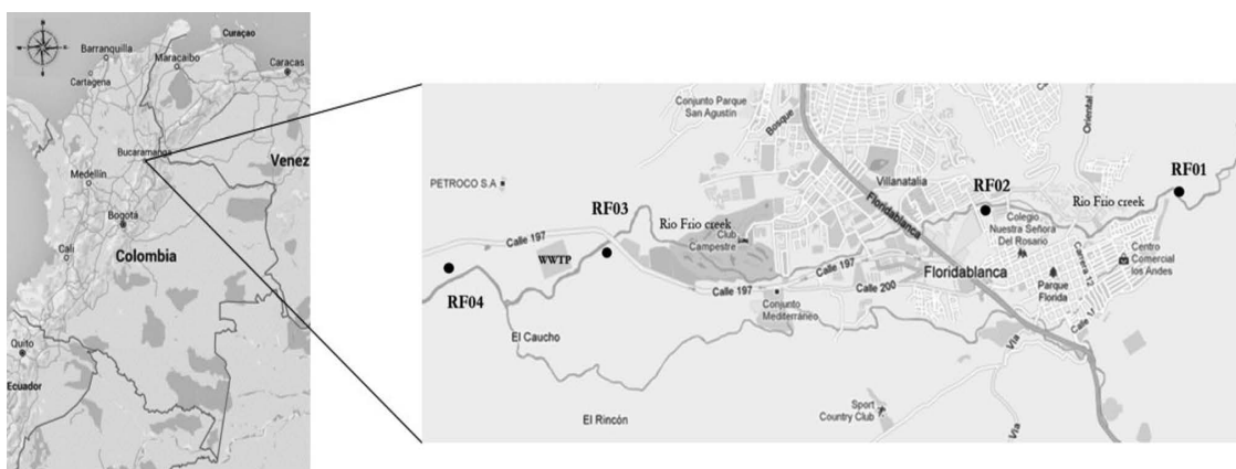
Figure 1. Río Frío (Bucaramanga-Santander-Colombia) sampling sites location. Source: Google Earth map (2016).
