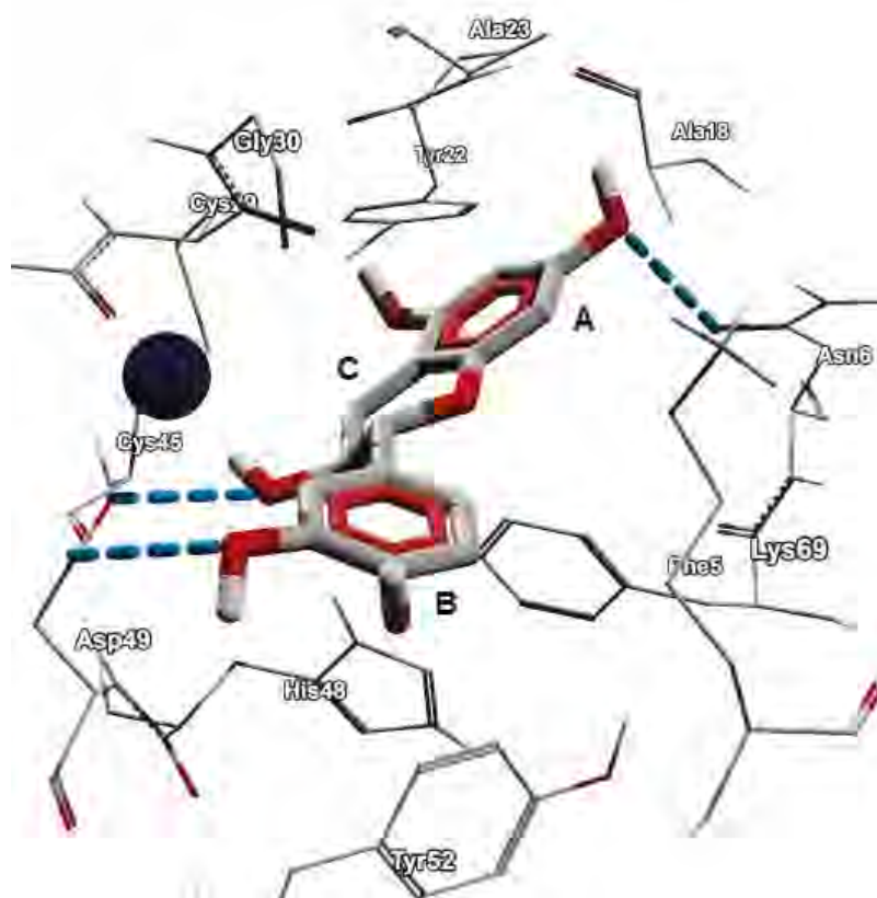
Figure 3. Molecular docking of (+)-catechin with a PLA 2 from the venom of Crotalus durissus terrificus . The blue sphere represents Ca 2+ . The dotted blue lines represent the hydrogen bonds. All the amino acids of the enzyme at a maximum distance of 3 Å are shown.
